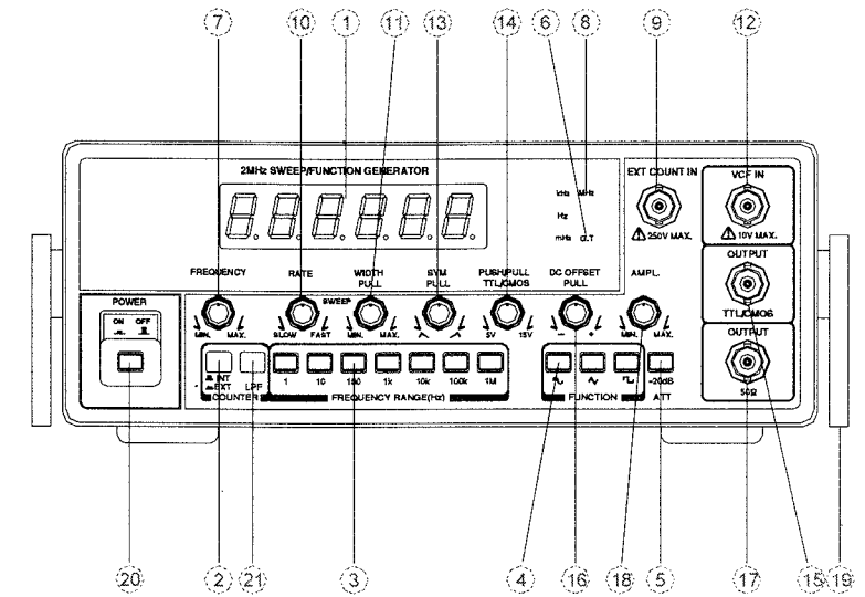
FIG 1-1. FRONT PANEL OPERATOR'S CONTROLS(8202,8203)
