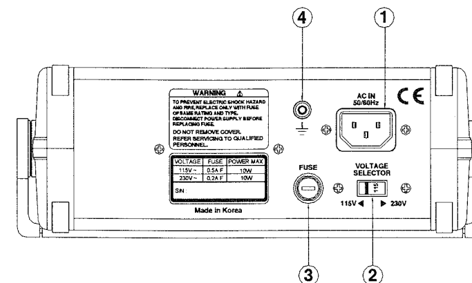
FIG 2-1. REAR PANEL(8202,8203)
