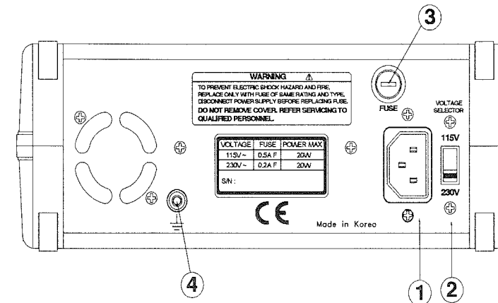
FIG 2-2. REAR PANEL(8205,8210)
