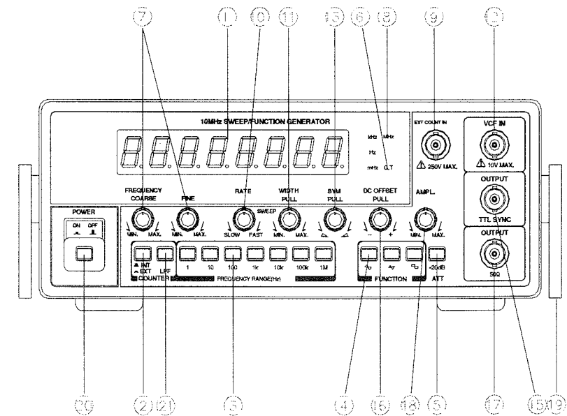
FIG 1-2. FRONT PANEL OPERATOR'S CONTROLS(8205,8210)
