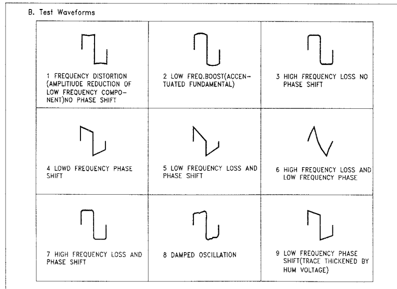
FIG 7. AMPLIFIER PERFORMANCE EVALUATION USING SQUARE WAVES.
